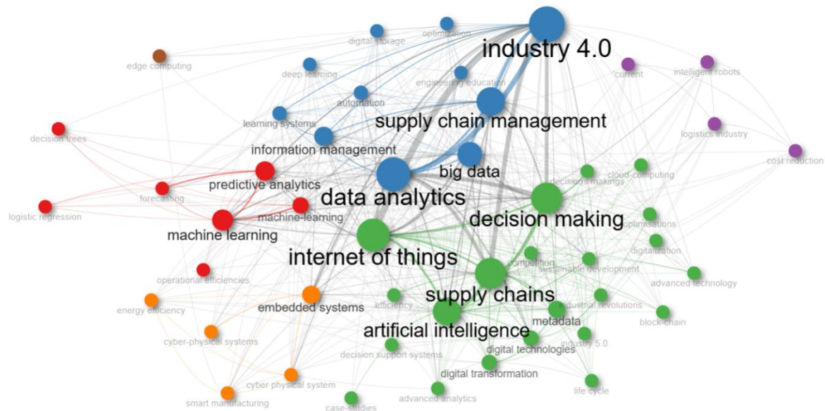
Figure 5: Co-occurrence network
